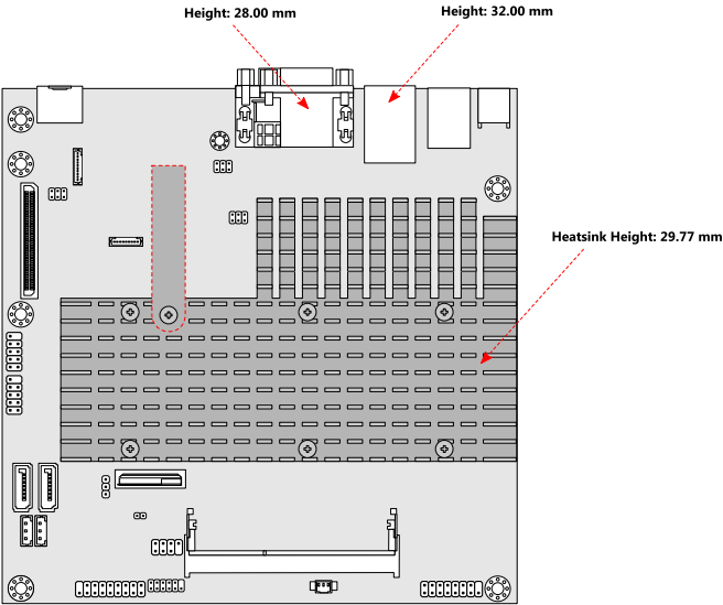
Figure 8: Height distribution of VB8004 mainboard (VB8004-12E SKU)
