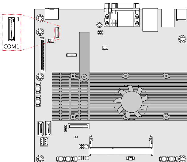
Figure 24: COM connector
