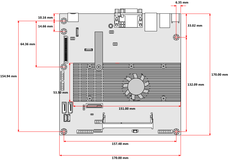
Figure 3: Dimensions of the VB8004 mainboard (VB8004-16 SKU)
