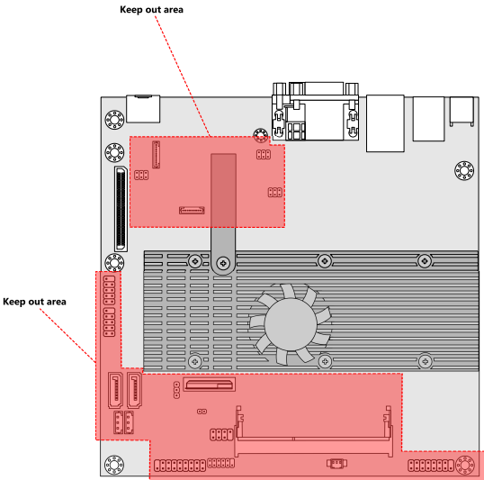
Figure 49: Suggested keep out areas for VB8004-12E SKU
