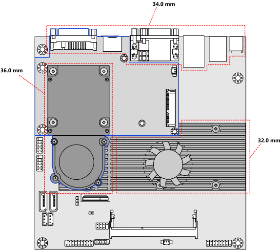
Figure 41: Suggested minimum internal chassis height for VB8004-6XS SKU
