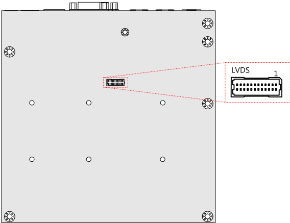
Figure 30: LVDS panel connector
