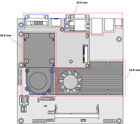
Figure 42: Suggested minimum internal chassis height for VB8004-16S SKU
