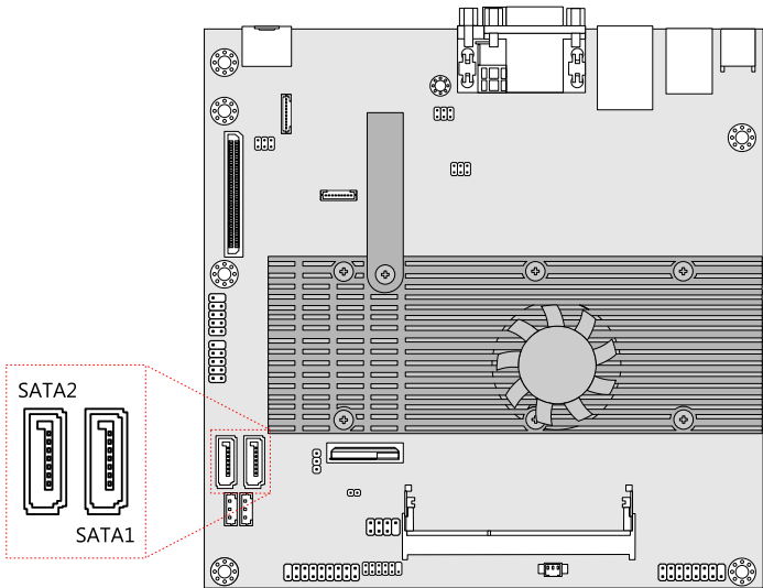
Figure 22: SATA connectors
